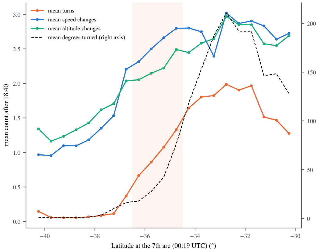
4. Manoeuvres by type against latitude — 7th arc (00:19 UTC)
