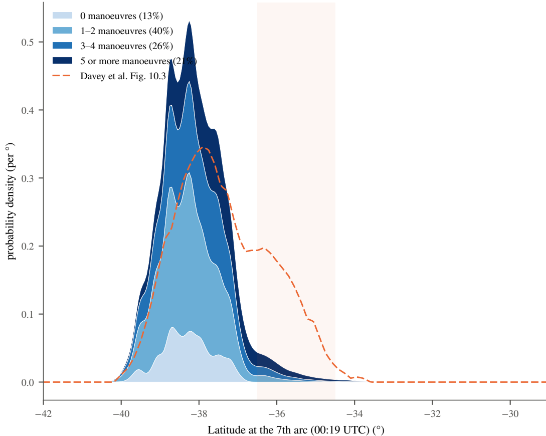
2. Latitude pdf split by complexity after 18:40 — 7th arc (00:19 UTC)
