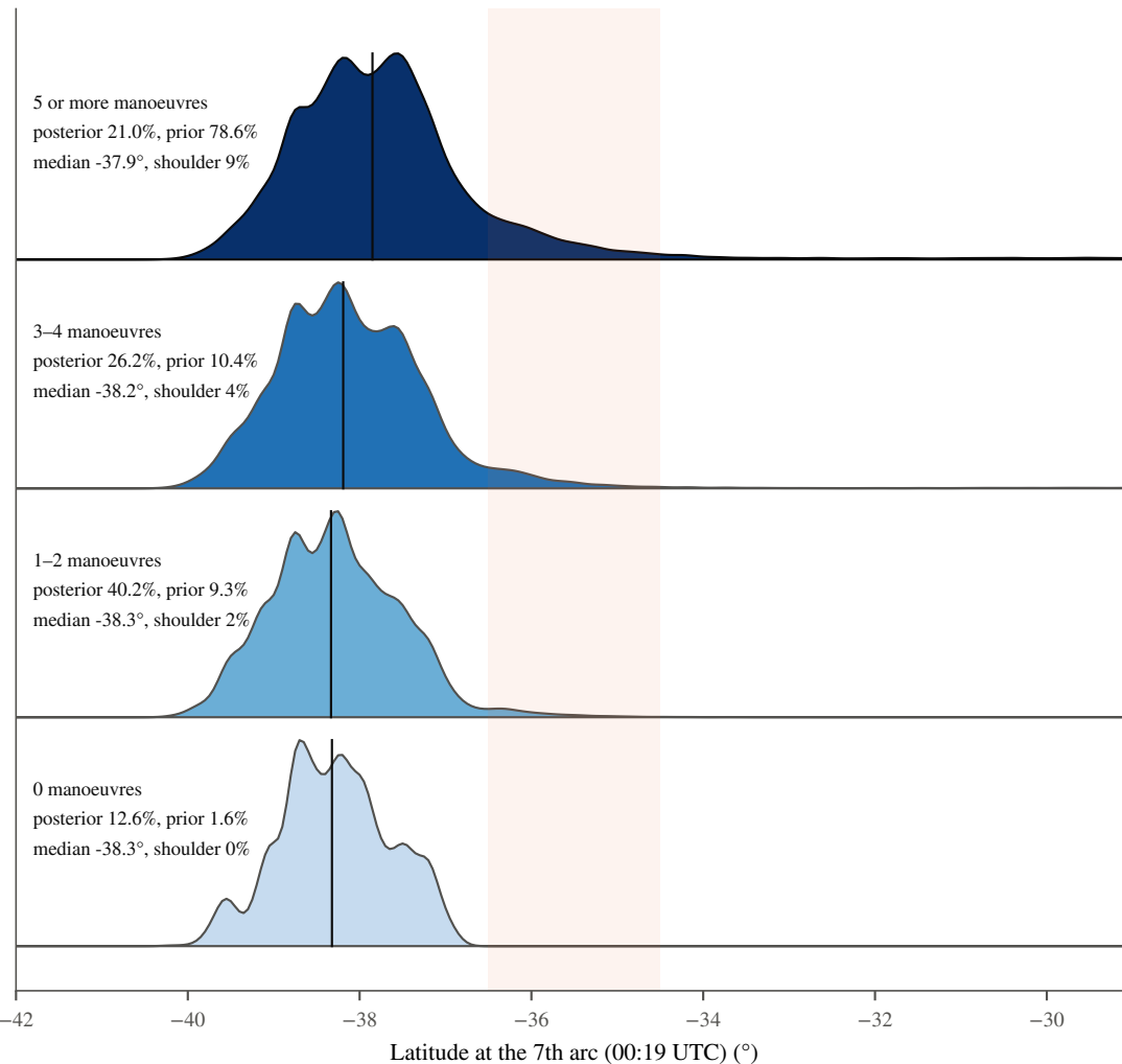
3. Latitude pdf of each complexity class (normalised) — 7th arc (00:19 UTC)
